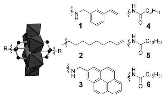
Scheme 1. Crystal structure of Mn-Anderson cluster [\text{MnMo}_6\text{O}_{18}((\text{OCH}_2)_3\text{C-R})_2]^{3-} with \text{MoO}_6 octahedra in dark gray and the central \text{MnO}_6 octahedron in light gray. Carbon atoms are depicted as black spheres and the residues R for compounds 1 to 6 are drawn as skeletal formulae. [20]
