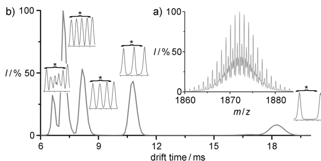
Figure 2. a) The mass spectrum for compound 1 for m/z 1860–1885 Da. b) The IM chromatogram for the deconvoluted peak envelope shown. The signals from left to right represent \{[(\mathbf{1})\text{TBA}_2]_n\}^- procession from n=5 to n=1 , with frames of the time-resolved mass spectrum for charge determination. Asterisk marks 1 amu.
