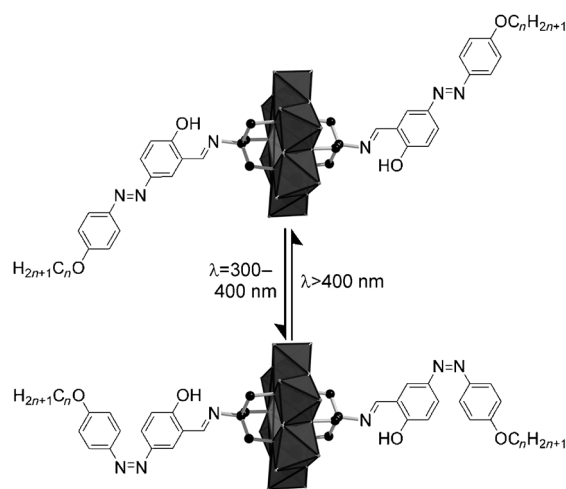
Scheme 2. Switching of photoresponsive Mn-Anderson cluster. Upon UV irradiation, the azo bond switches from trans to cis conformation. Under light irradiation, the bond switches back again. Three compounds ( 7 , 8 , and 9 with n = 8, 10 , and 12 ) were investigated.
