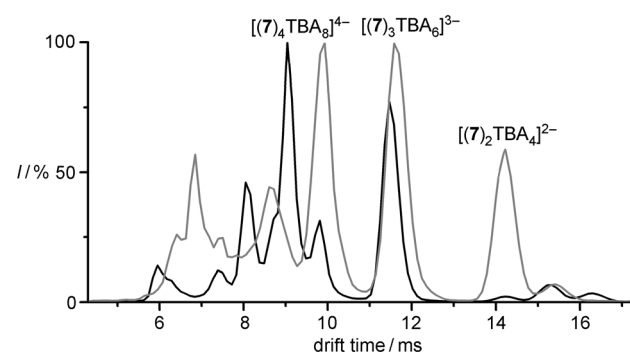
Figure 3. Comparison of the drift time graphs of the main envelope ( m/z = 2305\text{--}2320 \text{ Da} ) for the native compound 7 (black) and after UV irradiation (gray). The spectra were consistent for all three repeated cycles.
