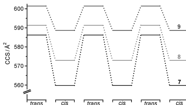
Scheme 3. Change in collision cross-section of dimers of compounds 7 , 8 , and 9 when switching between the trans and the cis conformation of the azo bond. The formula of the dimeric assemblies is [(\mathbf{X})_2\text{TBA}_4]^{2-} .
