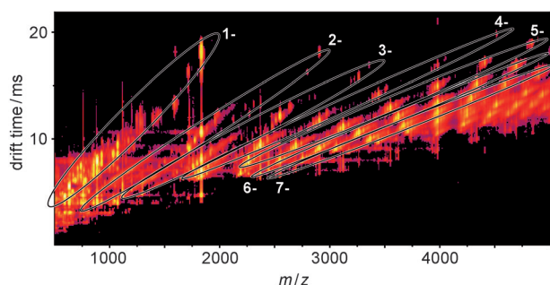
Figure 1. 2D IMS/MS spectrum of compound 1 . The diagonal lines of similarly charged species are encircled by ellipsoids and the charges of these species are given in white. (Background noise is filtered out for clarity; the original spectrum can be found in the Supporting Information.)
